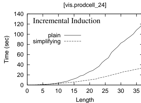
Fig. 4. Case study on incremental k -induction. The curve shows the progress of the temporal induction algorithm of TIP [ESb] running on the hardest example of Table 2. The graph plots the total execution time (y-axis) of all induction steps performed up to a certain length (x-axis). In this particular experiment, each step after length 25 takes more or less constant time.
